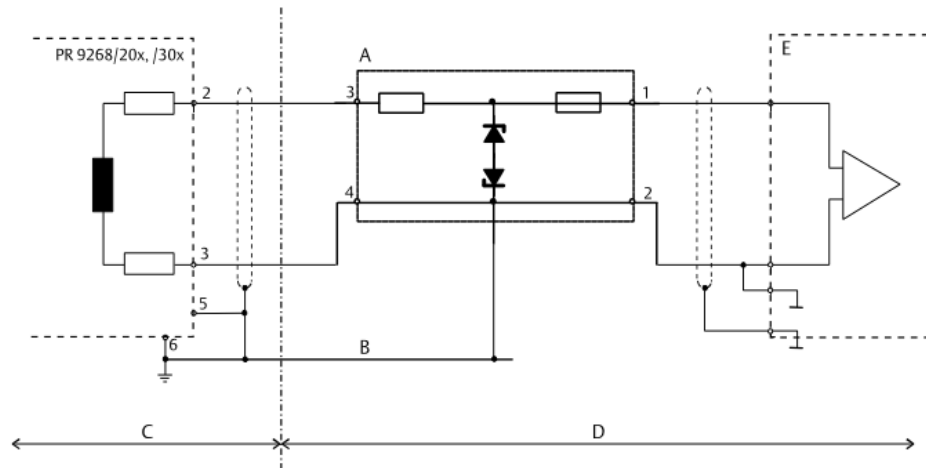
Figure 7-1: Connection example, intrinsically safe installation – PR 9268/20x-x00 and PR 9268/30x-x00
