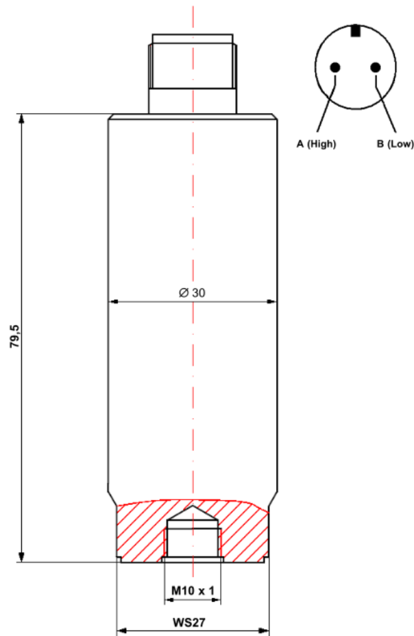
Figure 6-4: Dimensions – PE 9268/018-900
