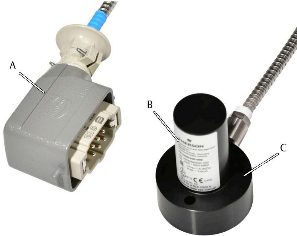
Figure 3-2: PR 9268/ 20x-x00 and PR 9268/30x-x00
