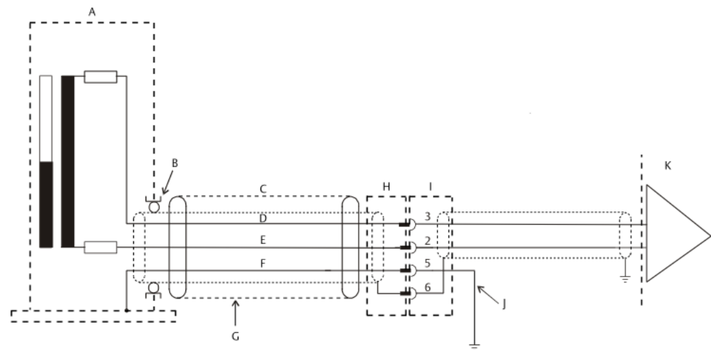
Figure 4-7: Connection diagram
