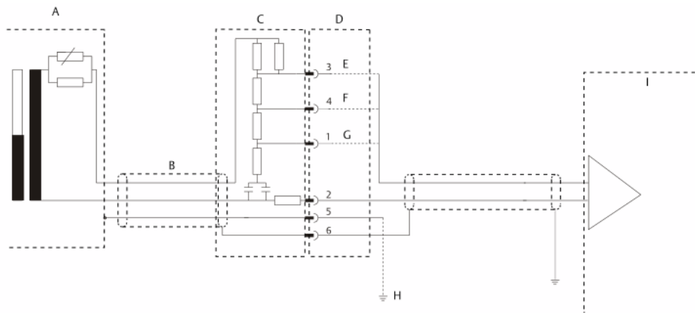
Figure 4-9: Connection diagram
