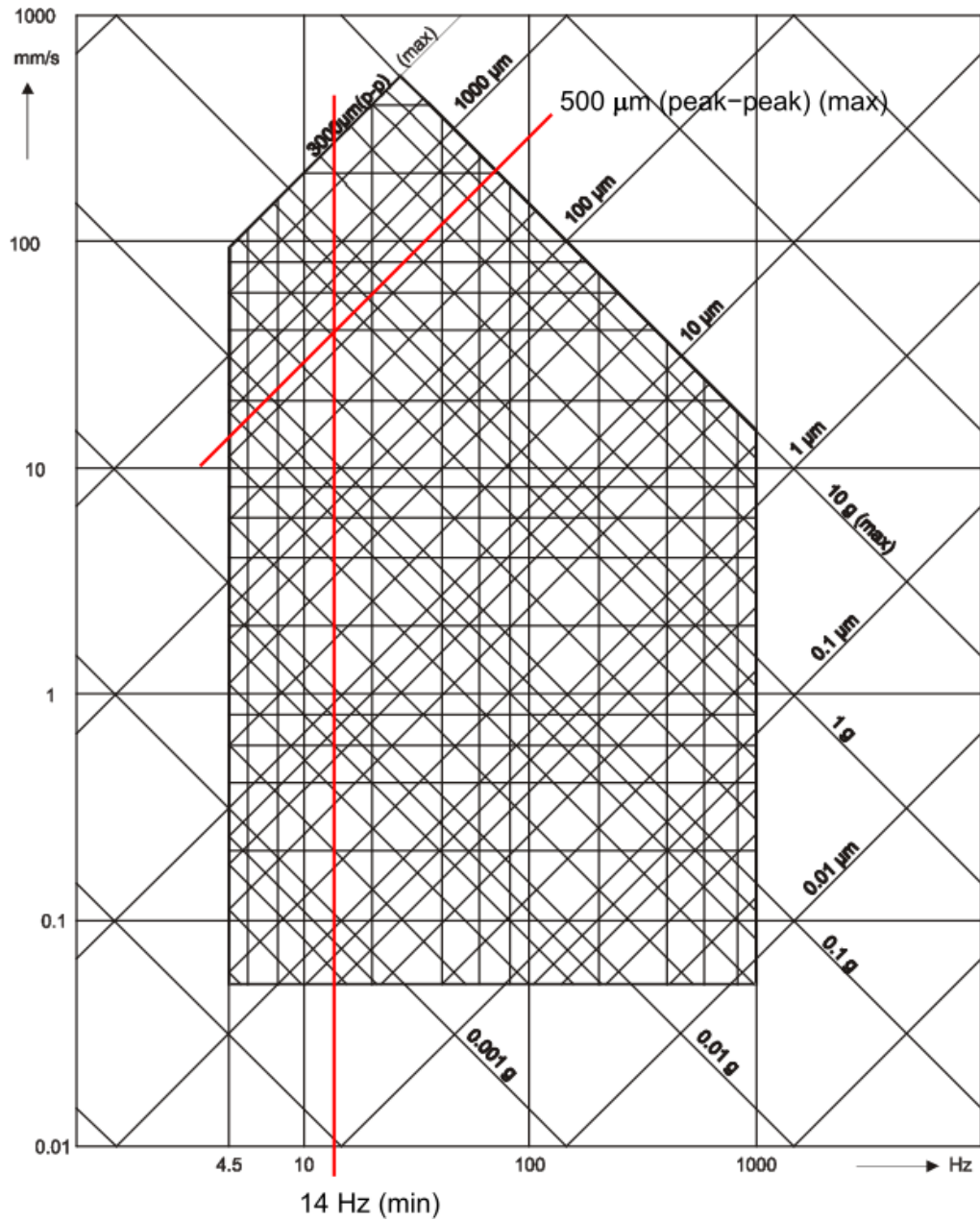
Figure 6-2: Nomogram operating range – PR 9268/01x-x00
