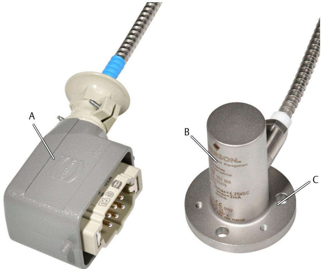
Figure 3-3: PR 9268/60x-000 and PR 9268/70x-000
