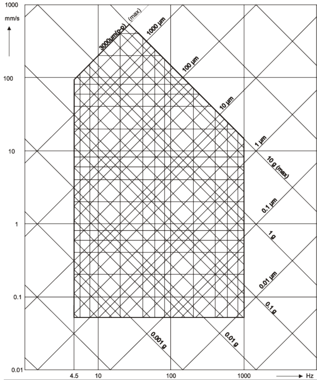
Figure 6-1: Nomogram operating range
