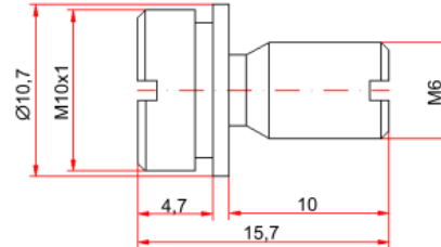
Figure 6-3: Dimensions – PR 9268/01x-x00
