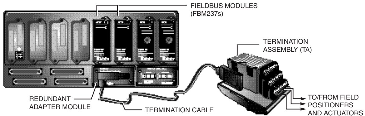
Figure 1. Redundant I/O Configuration
